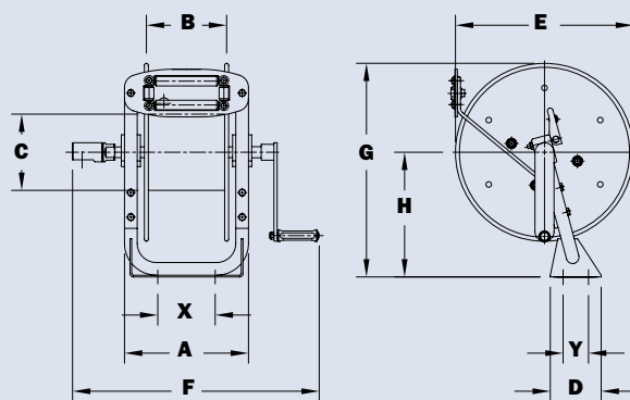
PWK-400 Wall mount with pivot
