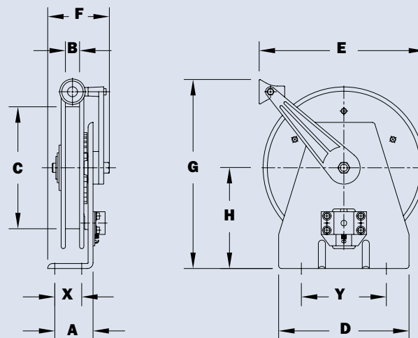
Model HGR50/HGR100/MHGR50 – HGR shown
